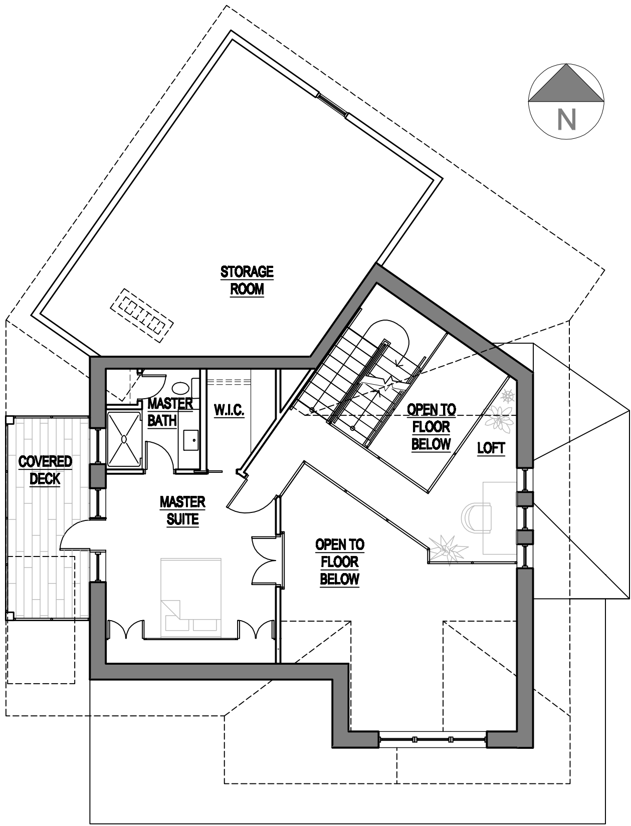
1 SECOND FLOOR PLAN A3 SCALE: 1/8"=1'-0"
