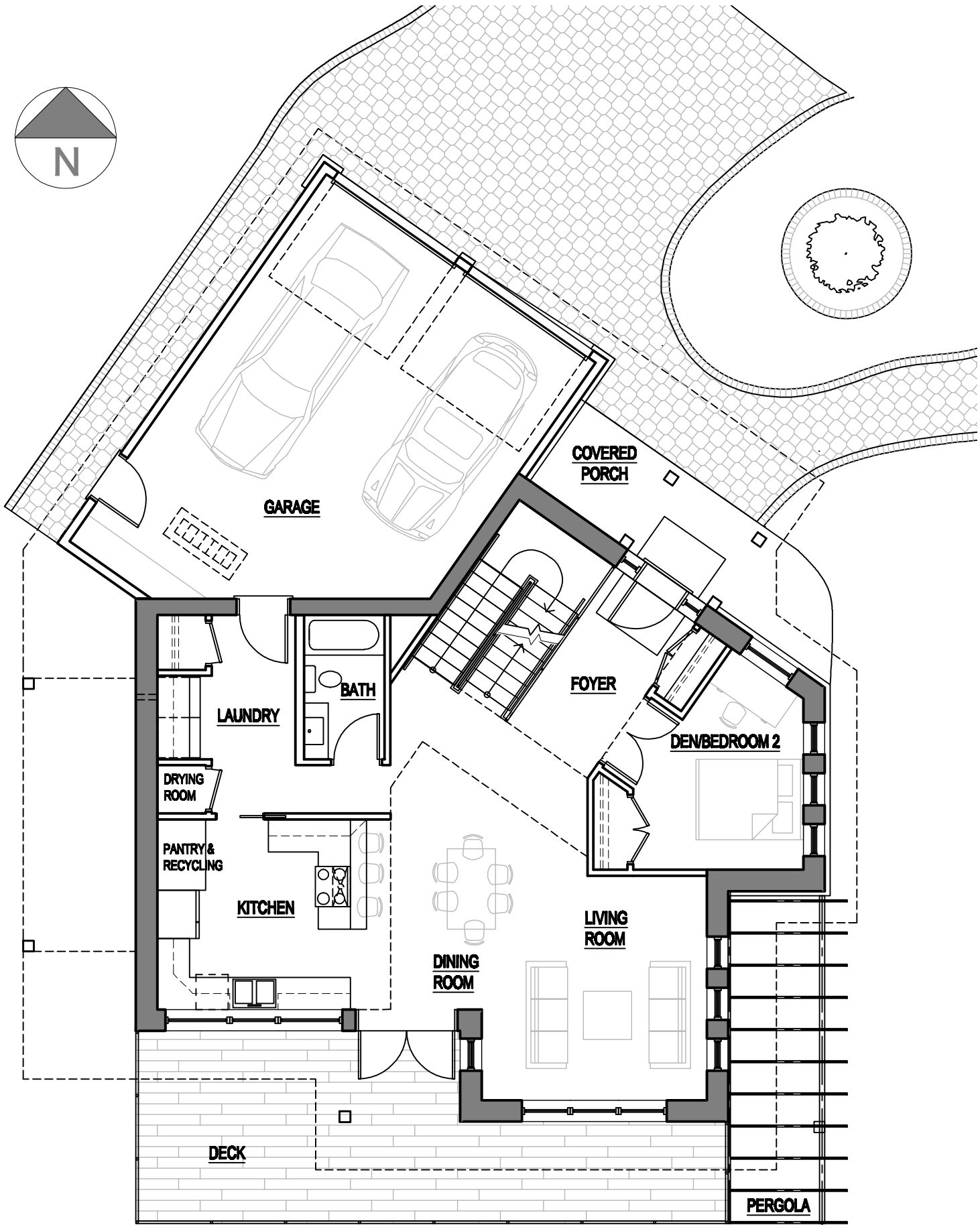
1 MAIN FLOOR PLAN A2 SCALE: 1/8"=1'-0"
